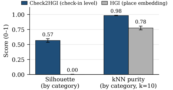
Fig. 3. Class separability of the representations on the ground-truth next-category labels (cosine silhouette; leave-one-out nearest-neighbor (kNN) purity, k=10 ), averaged over the five U.S. states. The check-in-level representation separates the seven categories; the place embedding does not.
